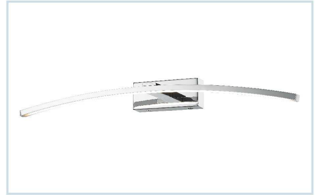
HLA-3612 (20W) Size : 824x50x100mm
