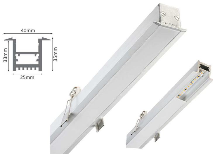
Model No.: HLL-4713 (40MM)
