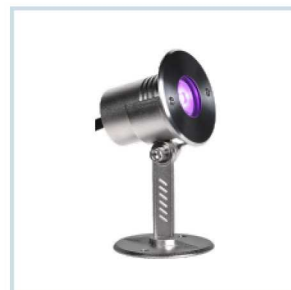
HLO-6502 (3W) - RGB Size : Ø68.5x132mm
