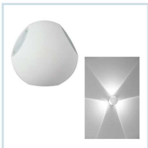
HLO-5364 (3x3W) Size : Ø100x88mm
