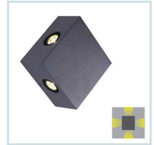
HLO-5354 (4x1W) Size : 100x100x52mm
